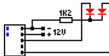
Intermitente LED
